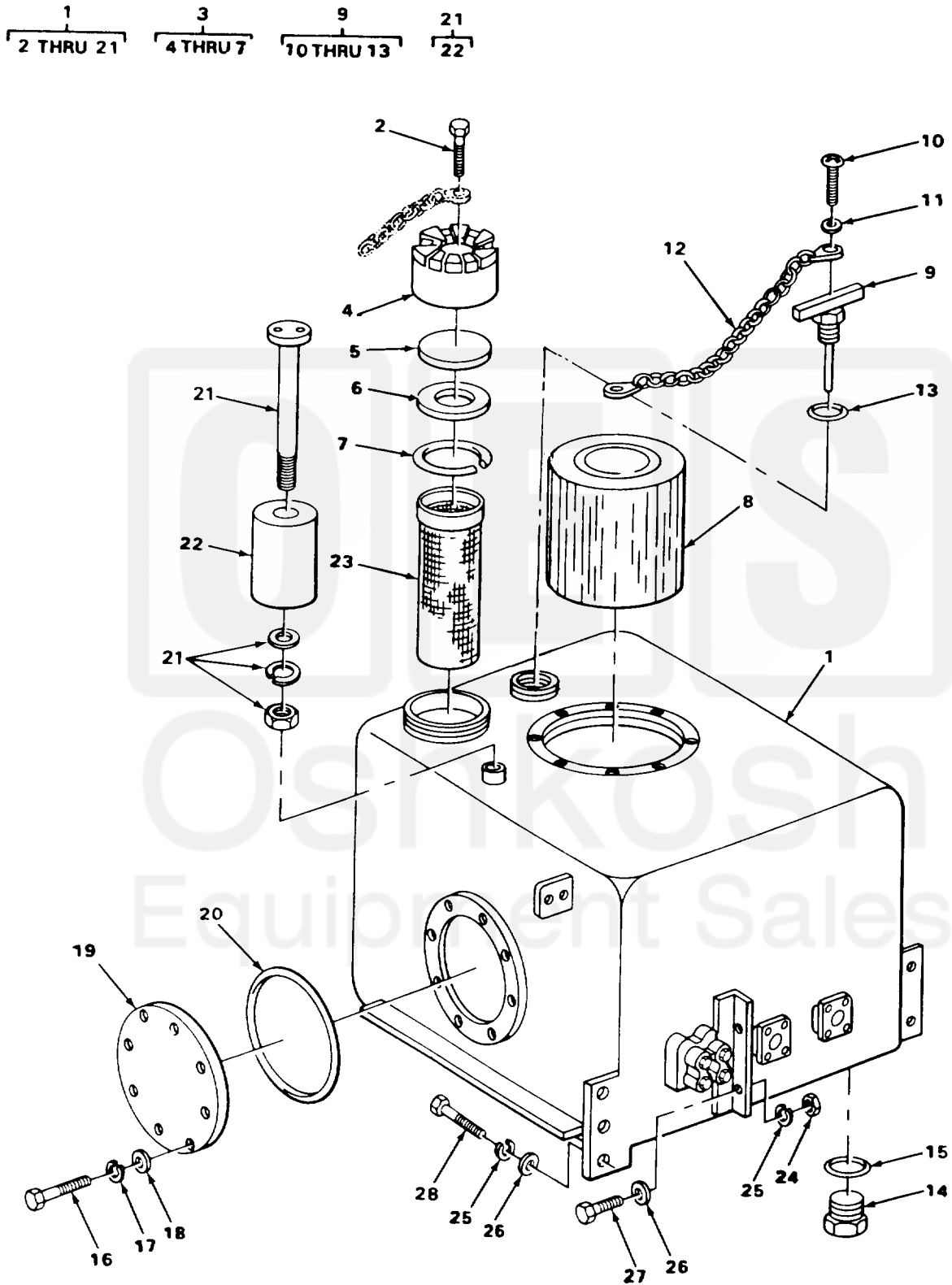
FIGURE 203. HYDRAULIC RESERVOIR
